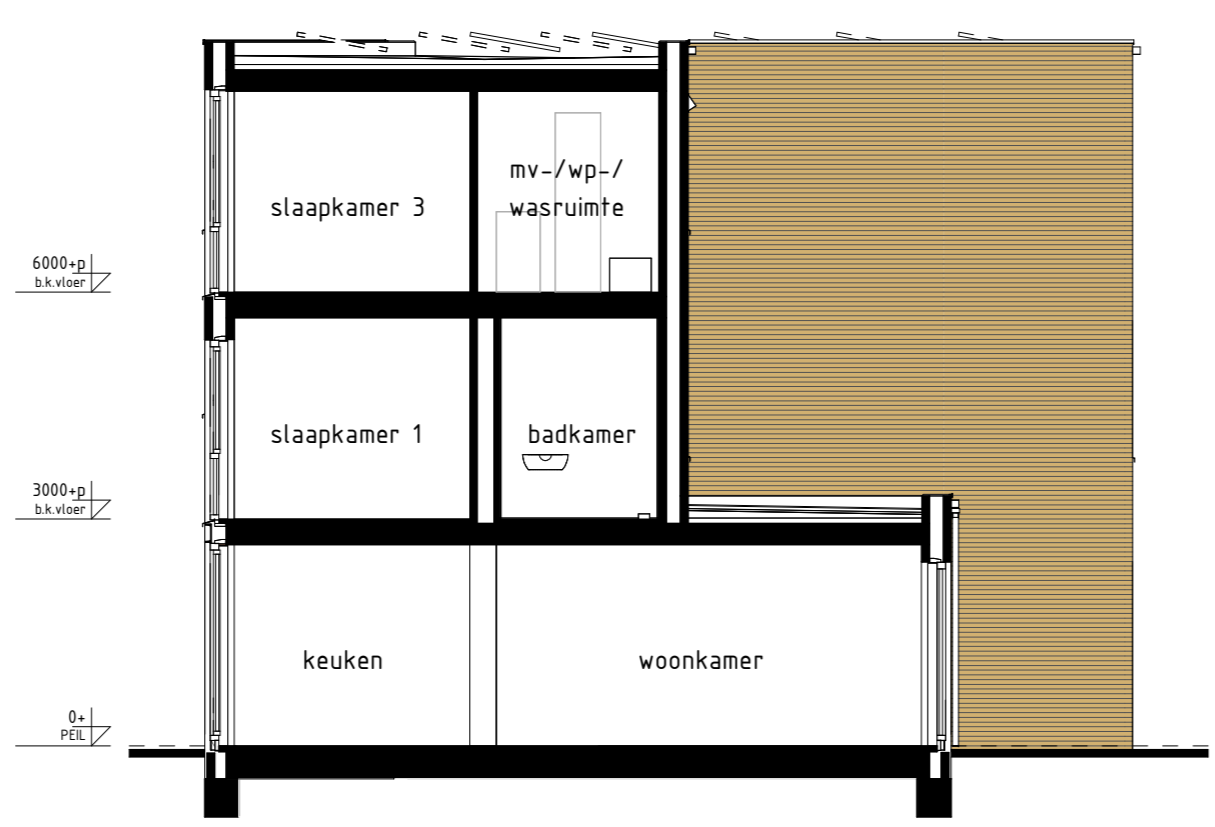
type F1sp, F2sp, F3sp bwnr get.:528, 529, 530, 531, 628, 629, 630, 631 DOORSNEDE 9D-9D
