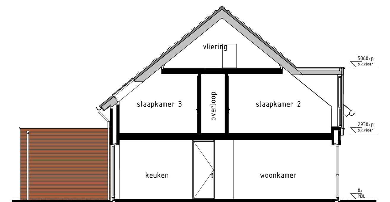
type H1sp, H1, G1, G2sp bwnr get.:11, 13 bwnr gesp.:12, 14 DOORSNEDE H1sp-H1sp 1:100
